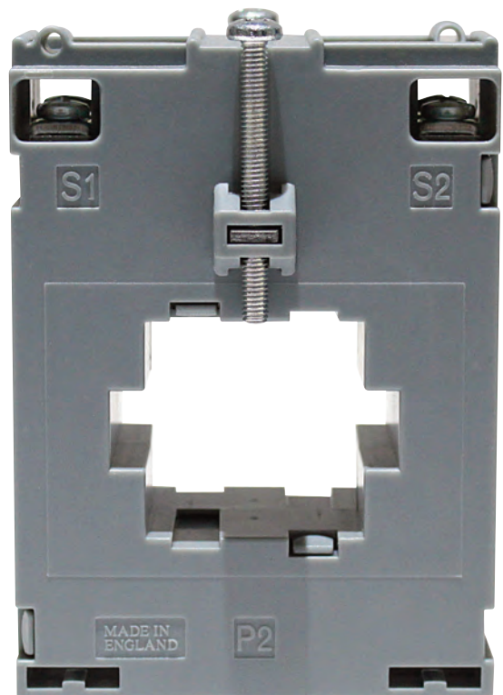
17 SERIES: TYPE 174 (Actual Size)
